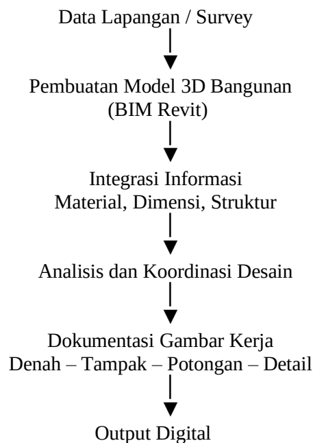
Gambar 2. Model 3D, Gambar Kerja, Quantity
