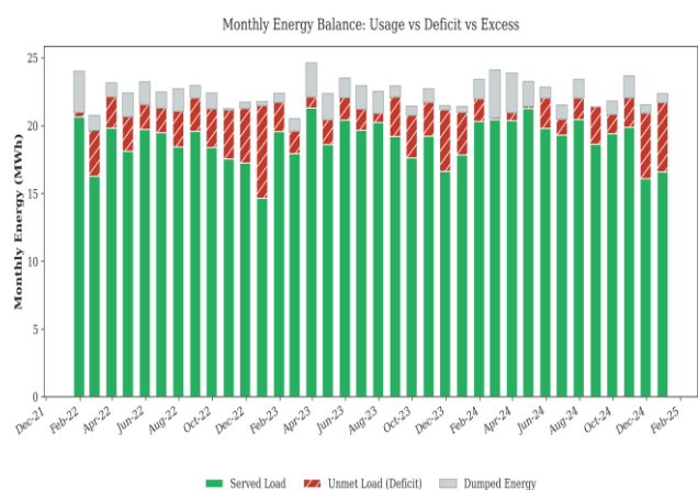
Figure 7. Monthly energy balance in 3 years
