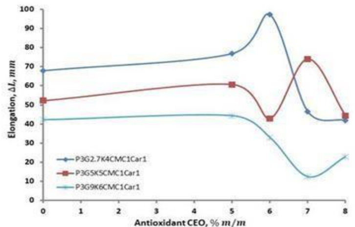
Fig. 16. Change in length (elongation, \Delta L ) in mm for Bruguiera gymnorrhiza fruit starch-based biodegradable plastics at various concentrations of antioxidants, CEO
