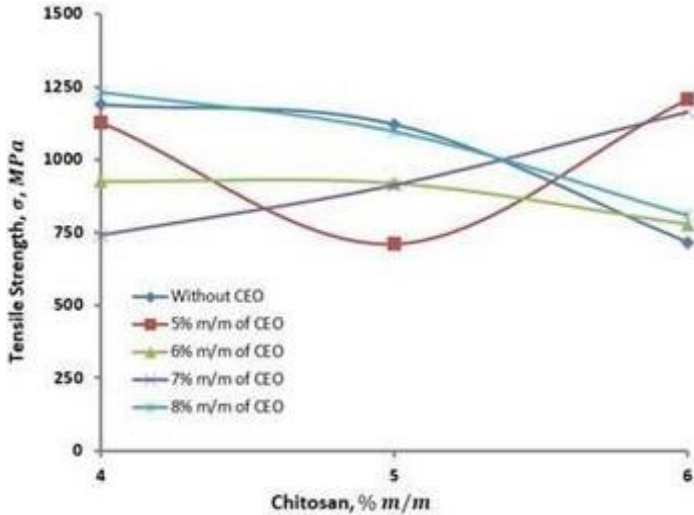
Fig. 9. The effect of the increase in chitosan concentration against the tensile strength ( \sigma ) of Bruguiera gymnorrhiza fruit starch-based biodegradable plastics 'without' and 'with' antioxidants CEO
