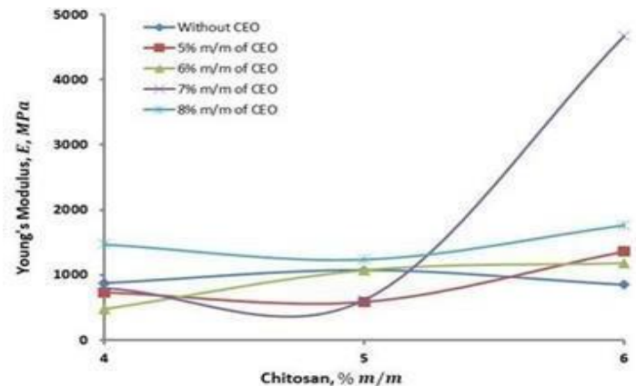
Fig. 12. The Effect of chitosan concentration on Young's Modulus (E) in MPa for Bruguiera gymnorrhiza fruit starch-based biodegradable plastics 'without' and 'with' antioxidant additives CEO
