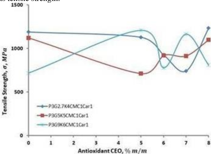
Fig. 10. Tensile strength ( \sigma ) in MPa for Bruguiera gymnorrhiza fruit starch-based biodegradable plastics at various concentrations of antioxidants, CEO
