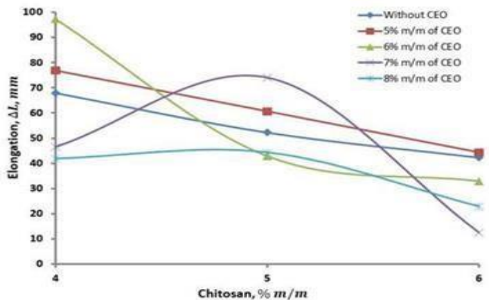
Fig. 15. Addition of chitosan against change in length ( \Delta L ) in mm for Bruguiera gymnorrhiza fruit starch-based biodegradable plastics 'without' and 'with' antioxidants, CEO
