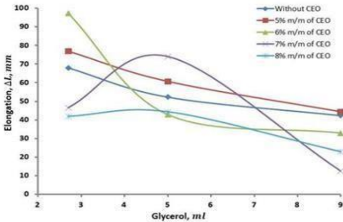
Fig. 14. Addition of glycerol in ml against change in length ( \Delta L ) in mm for Bruguiera gymnorrhiza fruit starch-based biodegradable plastics 'without' and 'with' antioxidants, CEO
