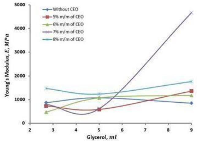
Fig. 11. The effect of the glycerol addition against the Young's Modulus (E) in MPa for Bruguiera gymnorrhiza fruit starch-based biodegradable plastics at various concentrations of antioxidants, CEO
