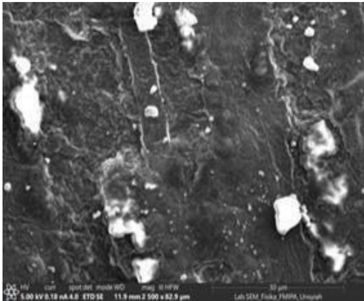
Fig. 6. A surface morphology and topography of biodegradable plastic sample with antioxidant agent: 8% (m/V) of CEO at 2500x optical magnification
