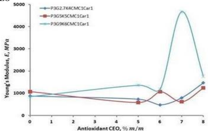
Fig. 13. Young's Modulus (E) in MPa for Bruguiera gymnorrhiza fruit starch-based biodegradable plastics at various concentrations of antioxidants, CEO.
