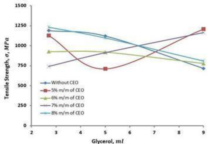
Fig. 8. The effect of the increase in glycerol concentration against the tensile strength ( \sigma ) of Bruguiera gymnorrhiza fruit starch-based biodegradable plastics ‘without’ and ‘with’ antioxidants CEO
