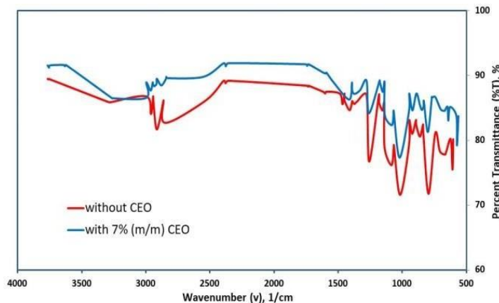
Fig. 4. The FT-IR spectral profiles for biodegradable plastic samples containing antioxidant agents or not
