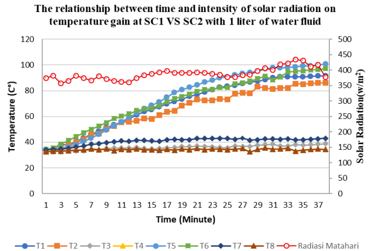
Fig. 5. The graph illustrates the relationship between time and solar radiation intensity with the temperature increase in the solar cooker system using 1 liter of water as the fluid.
