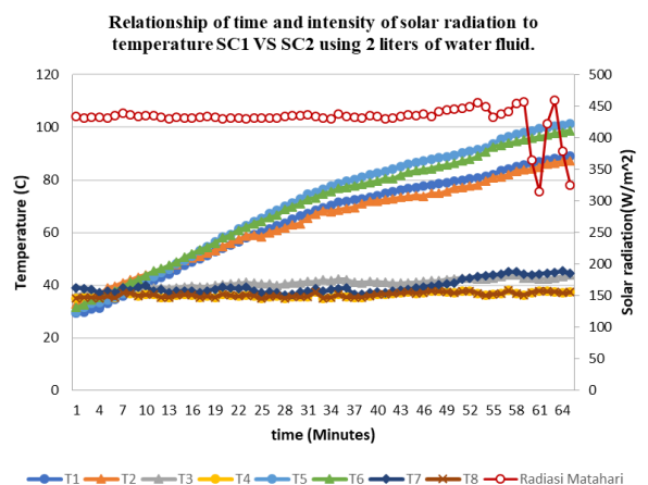
Fig. 13. Graph of the relationship between time and intensity of solar radiation on the temperature obtained by the solar cooker pan system using 2 liters of water fluid.
