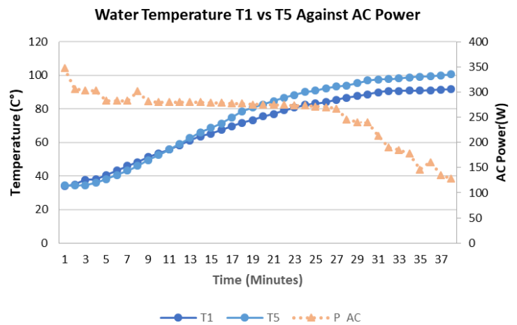
Fig. 8. Comparison chart of water temperature T1 vs T5 against AC power.
