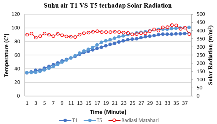
Fig. 6. Comparison graph of water temperature SC 1 (T1) vs water temperature SC 2 (T5) against solar radiation when cooking.
