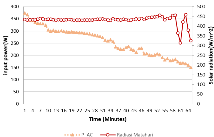
Fig. 15. Radiation power comparison graph.
