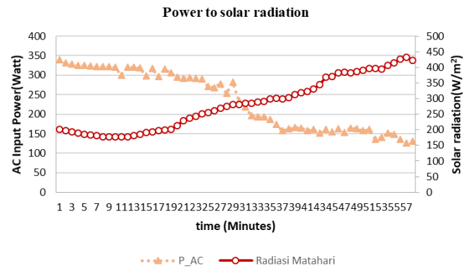
Fig. 12. AC Input output power and solar radiation graph.
