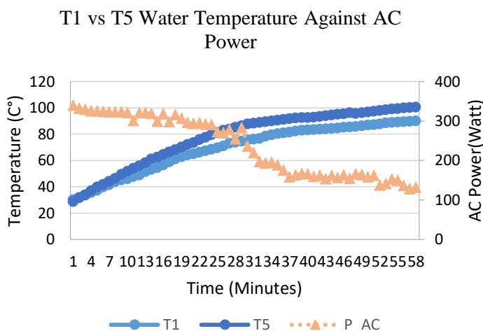
Fig 11. Comparison chart of T1 vs T5 temperature against AC power
