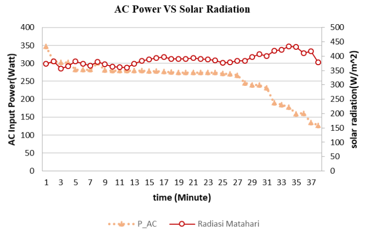
Fig. 7. Input power graph against solar radiation.
