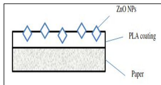
Gambar 2. Schematic illustration and structure of food packaging as paper coating from PLA-ZnO
