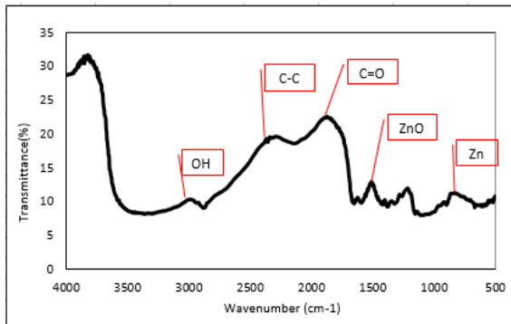
Gambar 3. Spectrum of FTIR ZnO Nanoparticle
