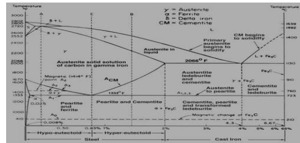
Gambar 1. Diagram Fasa[6]
