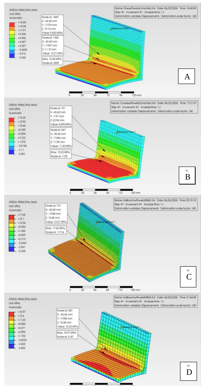
Fig. 12. Chamfer contour result based on method and mesh; (A) IIW LSE Fine, (B) IIW LSE Coarse (C) Haibach Fine, (D) Haibach Coarse
