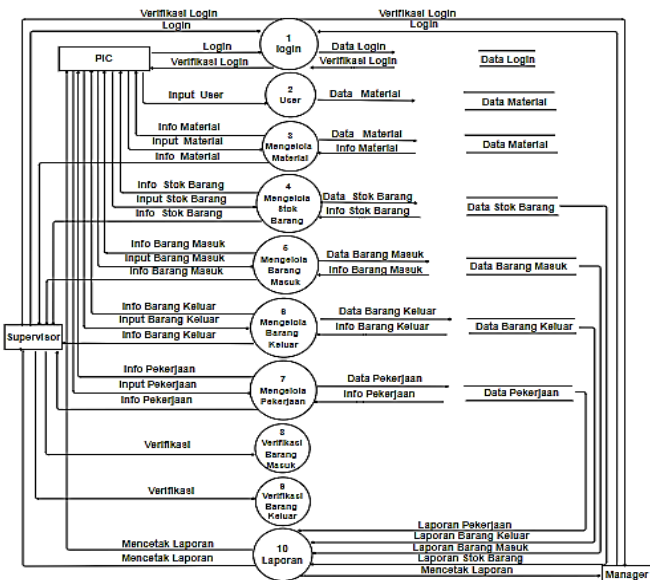
Gambar 2. DFD Level 0
