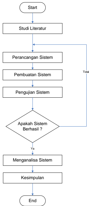
Gambar 1 Flowchart
