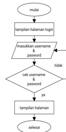
Gambar 3. Flowchart Login
