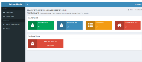
Gambar 22. Halaman Dashboard
