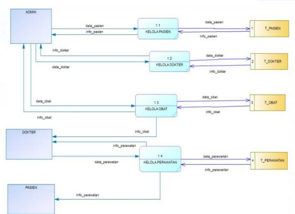
Gambar 4. DVD Level 0
