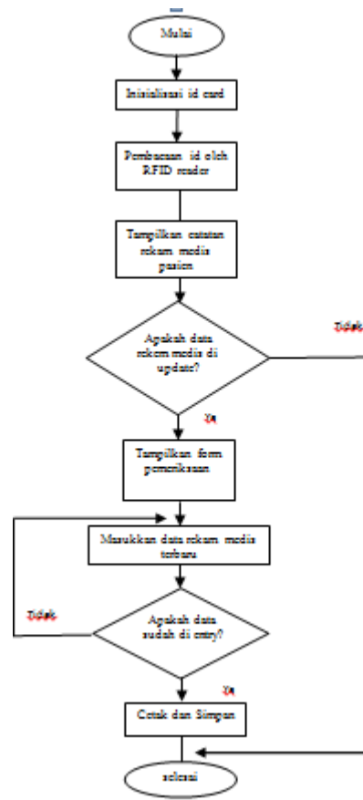
Gambar 2. Flowchart Sistem
