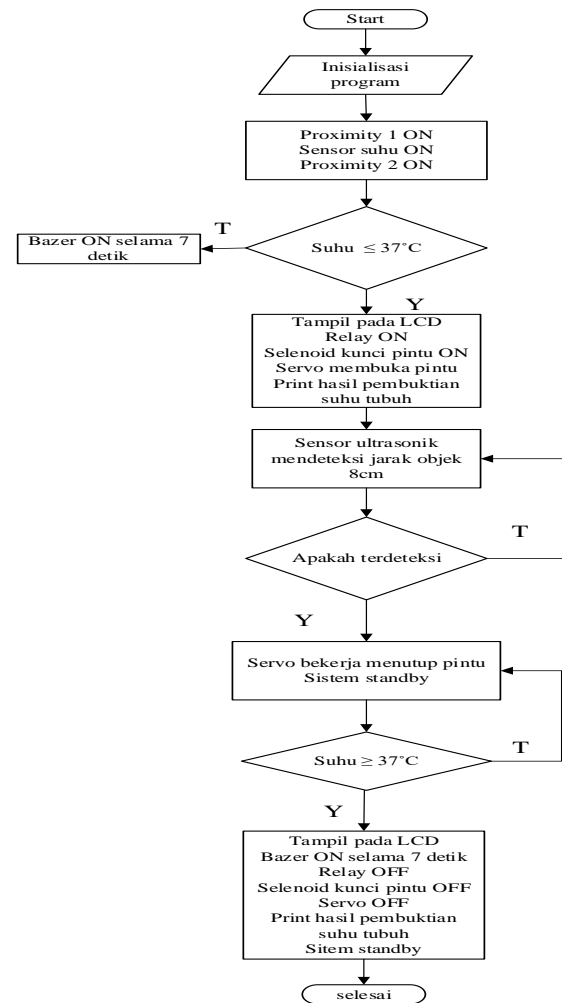
Gambar 8. Flow Chart Sistem
