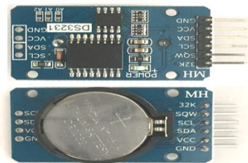
Gambar 4 Modul RTC
