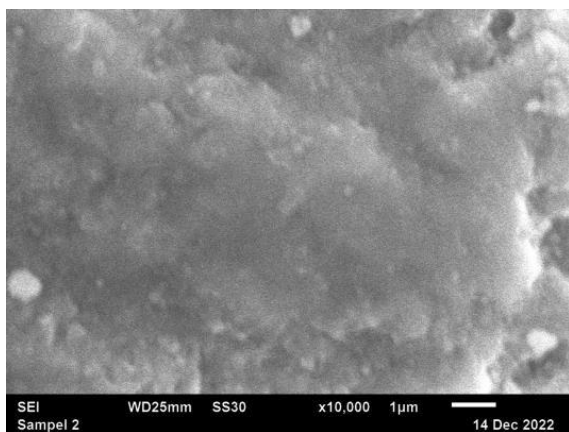
Figure 3.5 SEM test results of carbon steel samples using 40 ppm inhibitor
