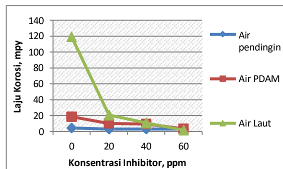
Figure 3.1 Effect of zinc phosphate base inhibitor concentration on corrosion rate
