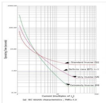
Gambar 2. Tipe karakteristik Overcurrent Relay invers
