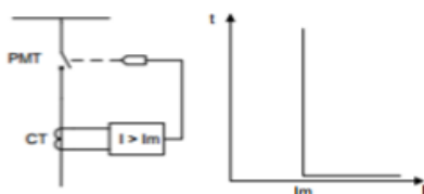
Gambar 4. Karakteristik OCR instantaneous time
