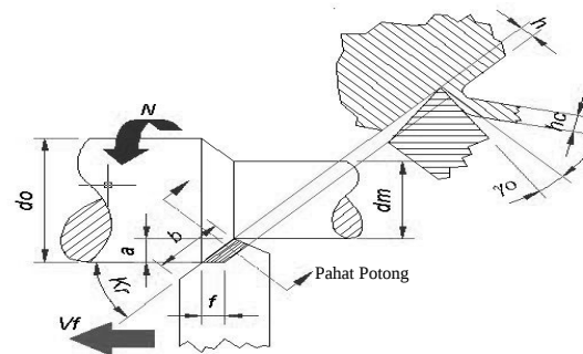
Gambar 1. Proses Bubut[2]
